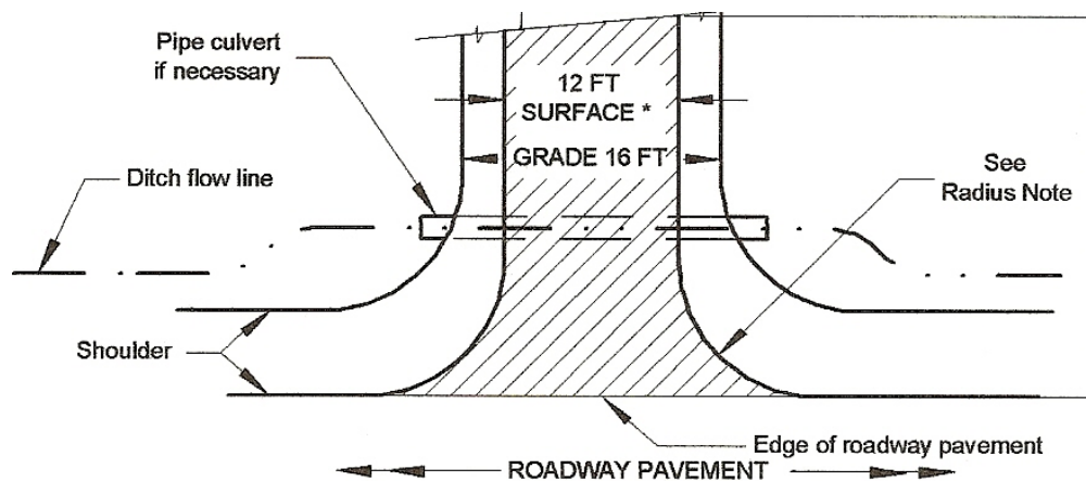
FIGURE 9 – PRIVATE ENTRANCE DETAIL
